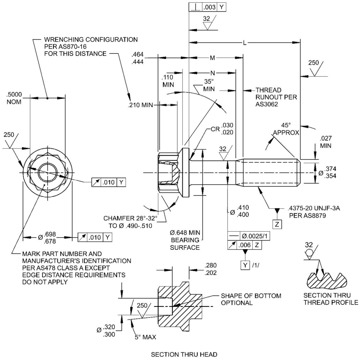
FIGURE 1 - BOLT
